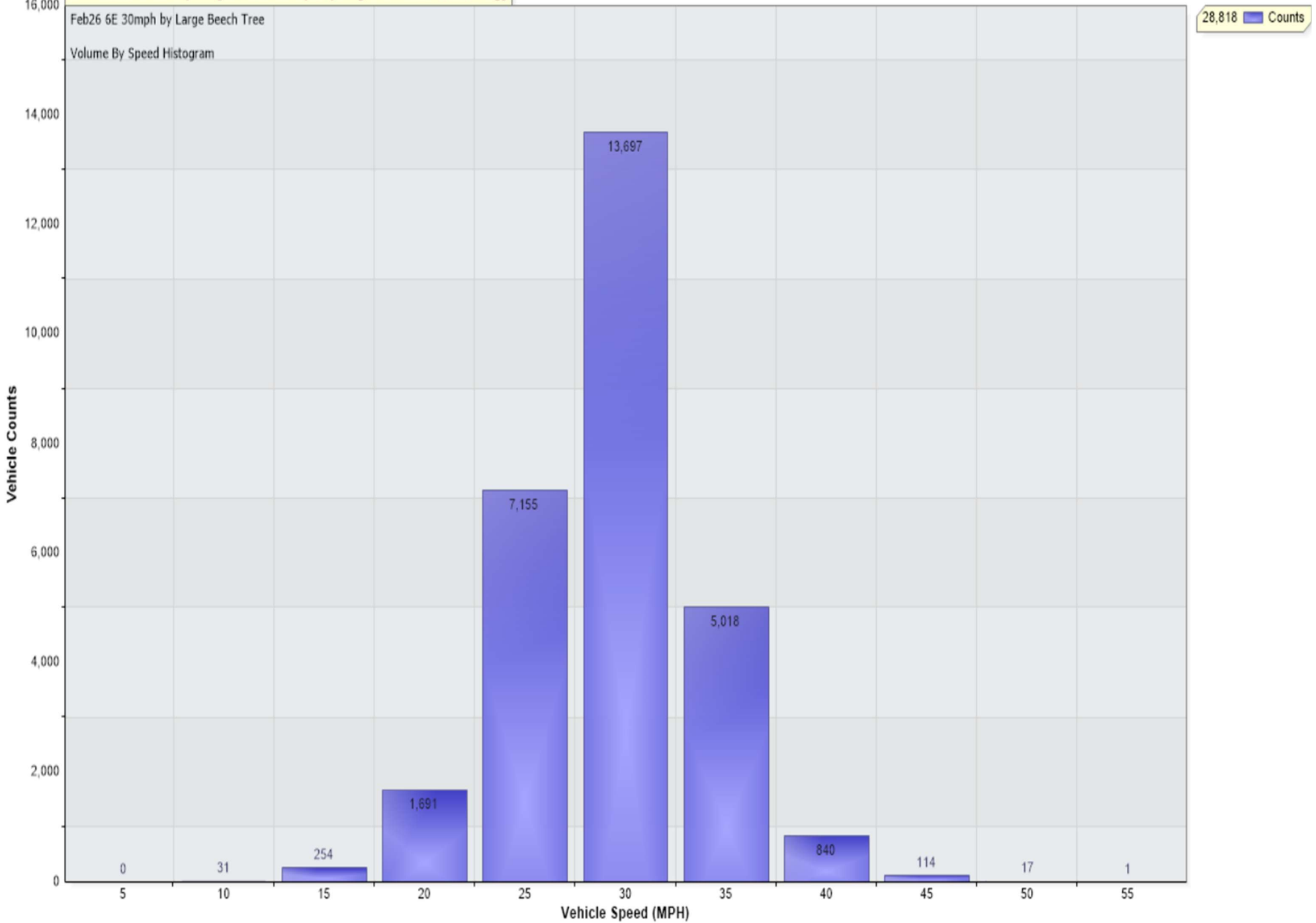
Vehicle Counts Vs. Speed [Feb26 6E 30mph by Large Beech Tree: Incoming]
