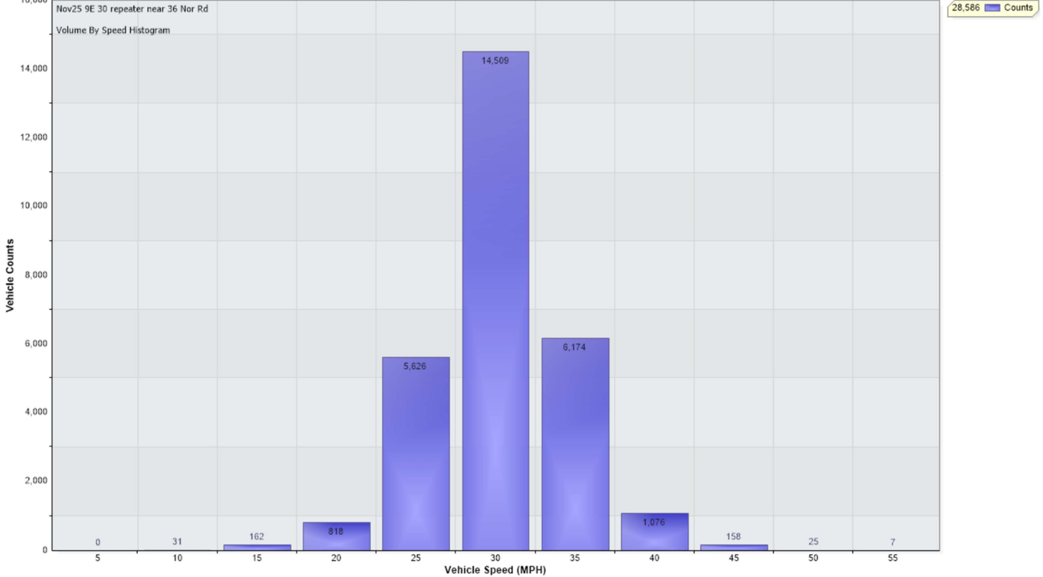
Vehicle Counts Vs. Speed [Nov25 9E 30 repeater near 36 Nor Rd: Incoming]
