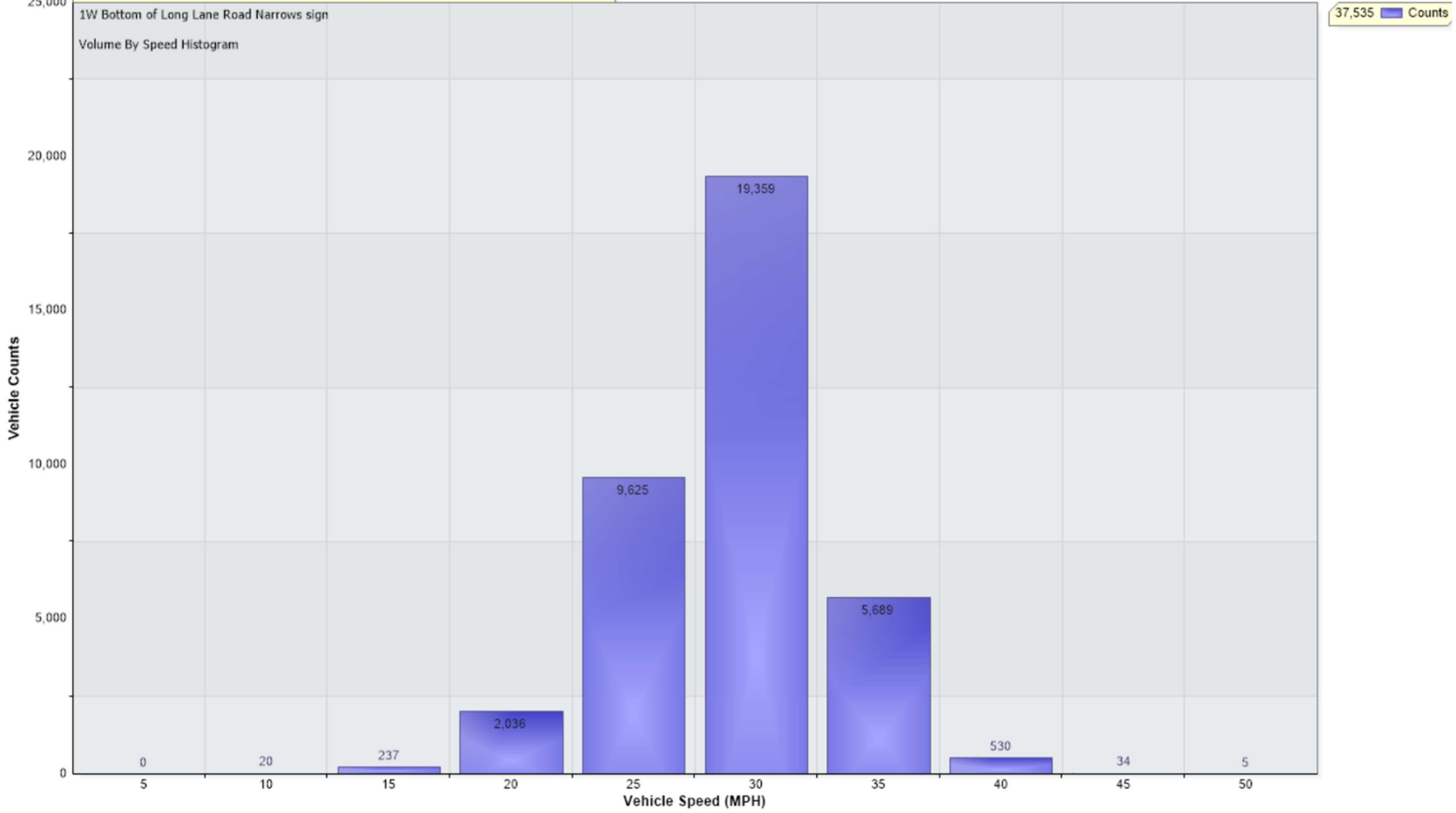
Vehicle Counts Vs. Speed [1W Bottom of Long Lane Road Narrows sign : Incoming]
