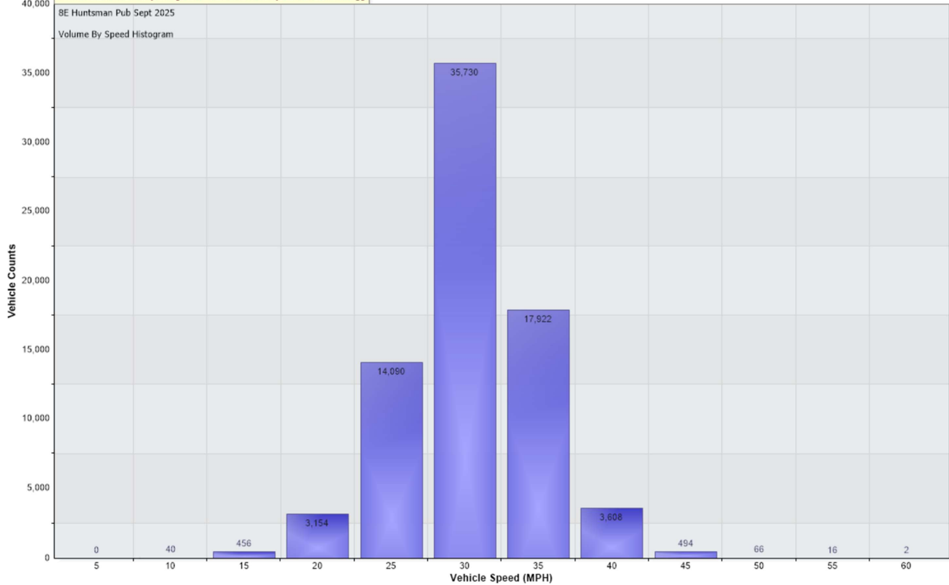
Vehicle Counts Vs. Speed [8E Huntsman Pub Sept 2025: Incoming]
