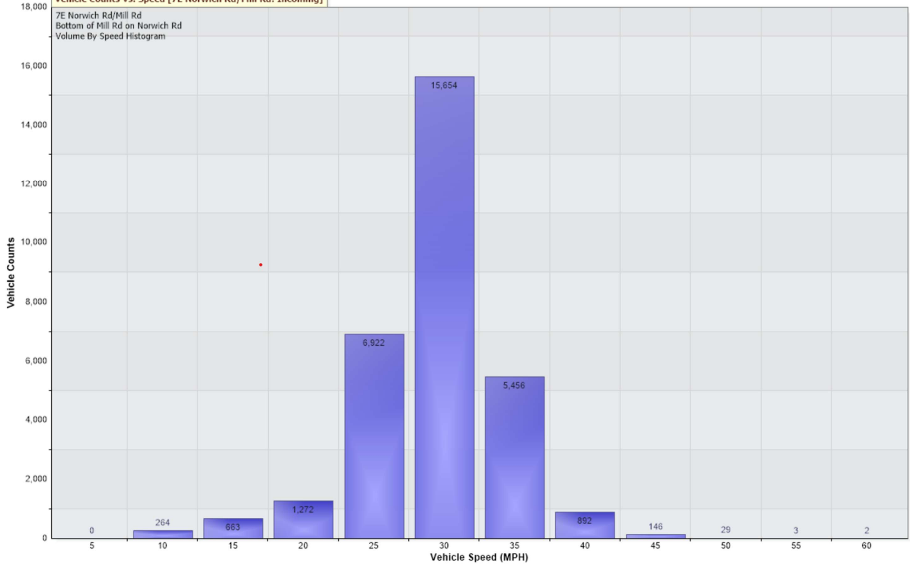
Vehicle Counts Vs. Speed [7E Norwich Rd/Mill Rd: Incoming]
